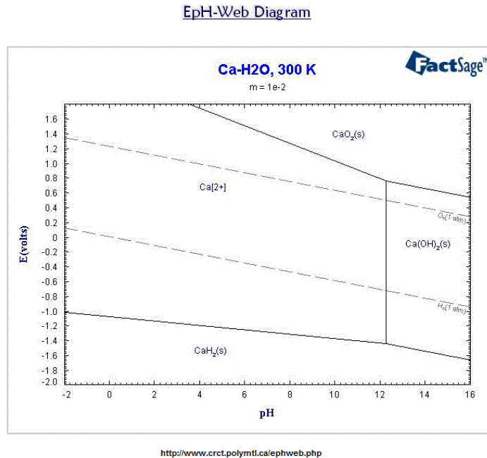
Figure 6: Marine corrosion of calcium based coral reefs and E-pH (Pourbaix) diagram for Calcium Based Corrosion
