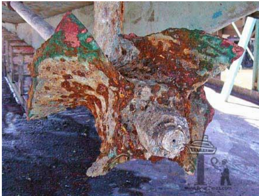
Figure 2: Accelerated marine corrosion due to stray electrical currents
