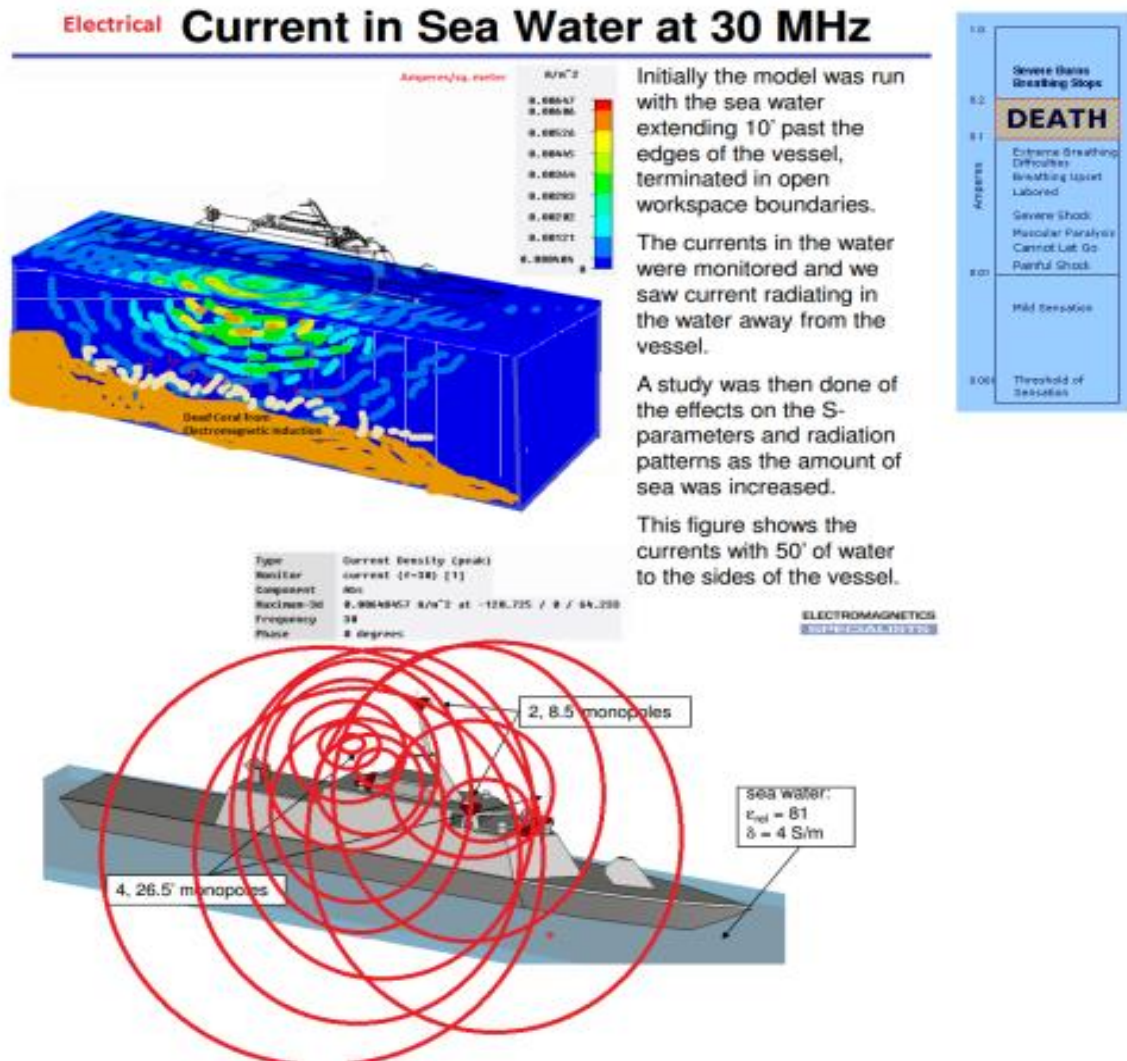
Figure 3: EM Simulation showing electrical currents induced in seawater due to EM Radiation from antennas
