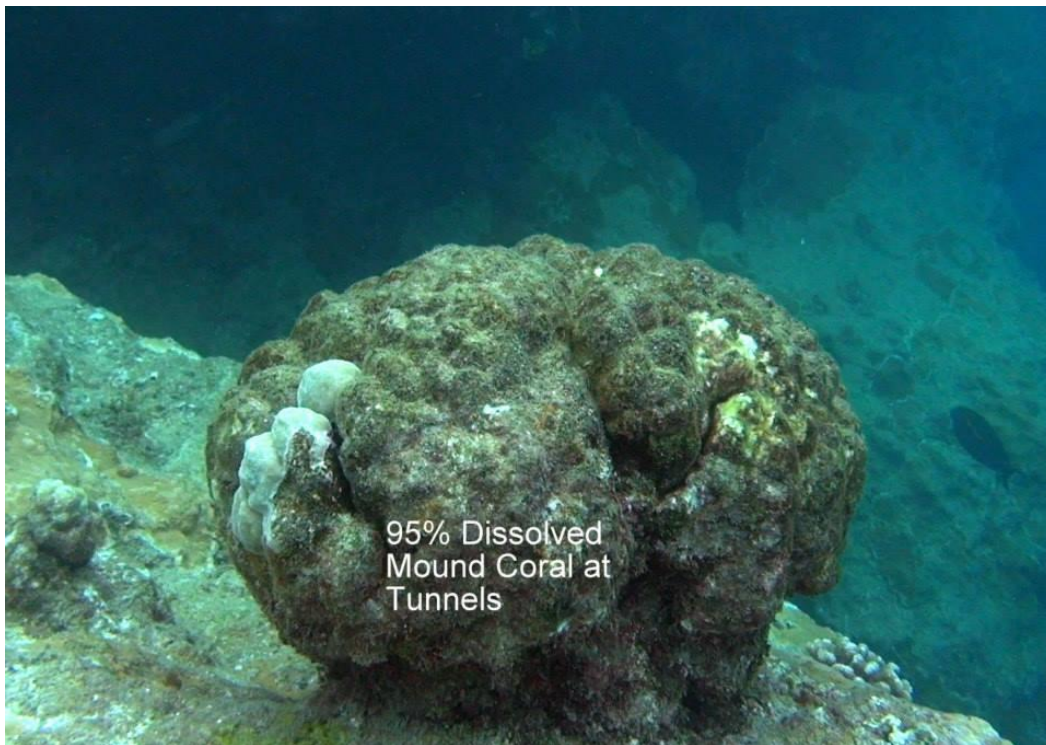
Figure 10: This mound coral structure is showing signs of accelerated corrosion below high power high gain antennas and radars in Kauai, HI
